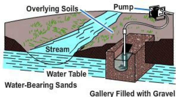
Figure 5-8 — Gravel filled gallery intake.
