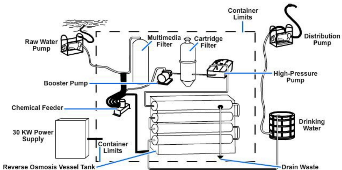
Figure 5-13 — Water flow through the 600 gph ROWPU.
