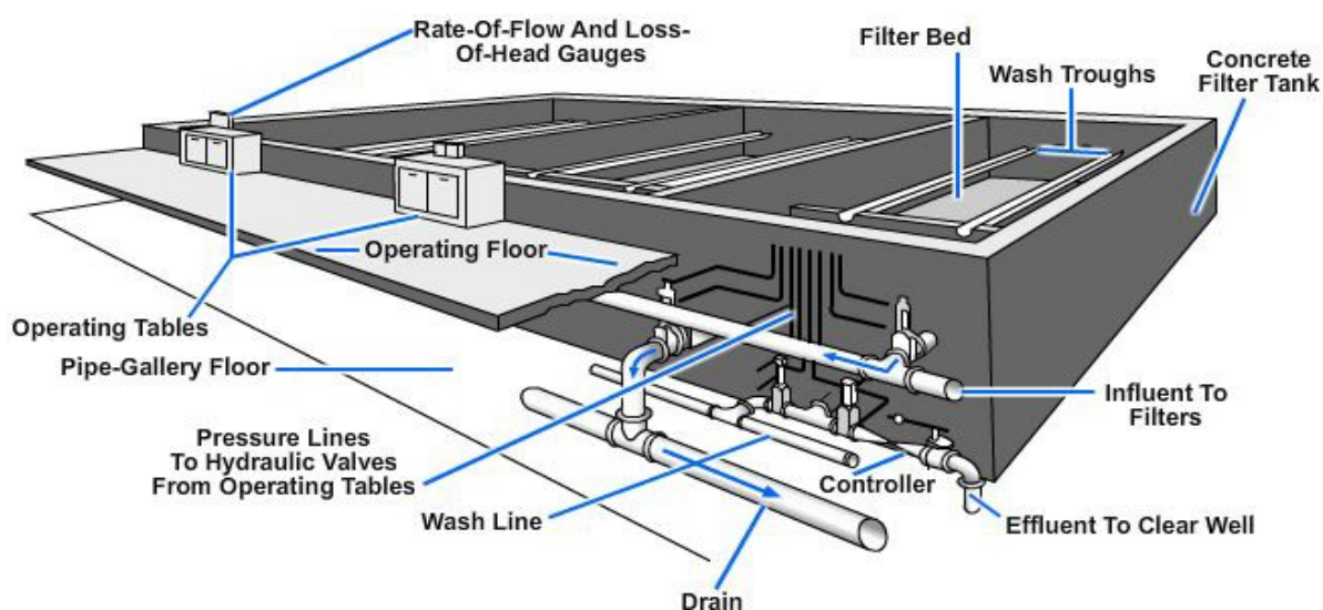
Figure 9-15 — Types of gravity filters.
