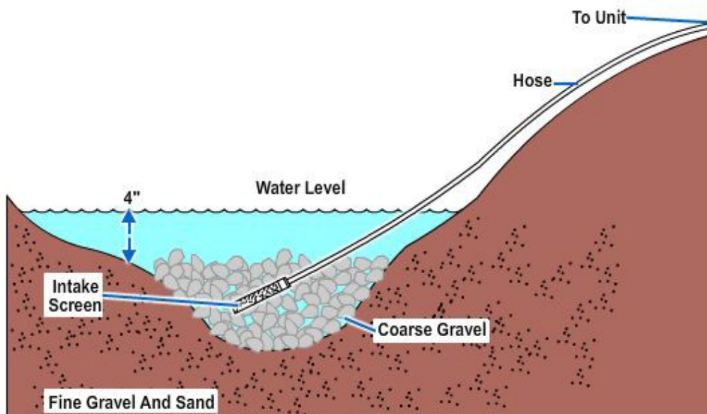
Figure 5-6 — Methods for securing a surface intake.
