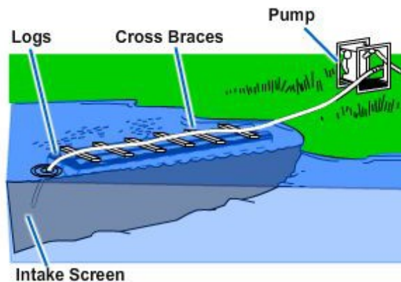
Figure 5-7 — Float type surface intake.
