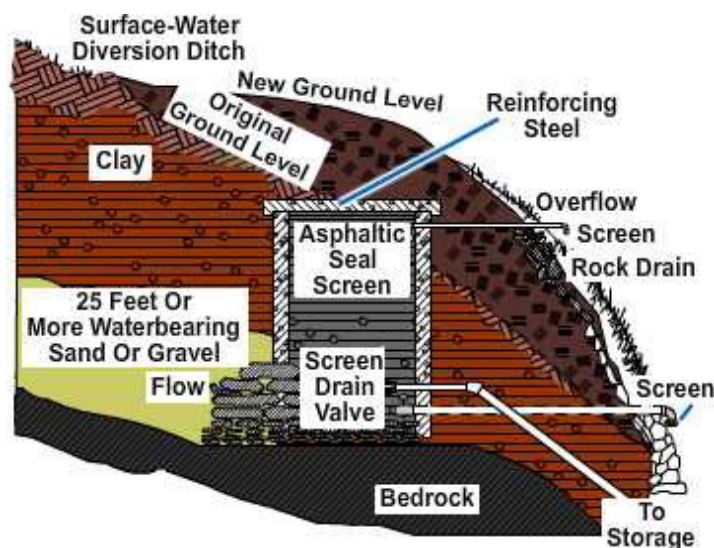
Figure 5-9 — Protection of spring from surface contamination.
