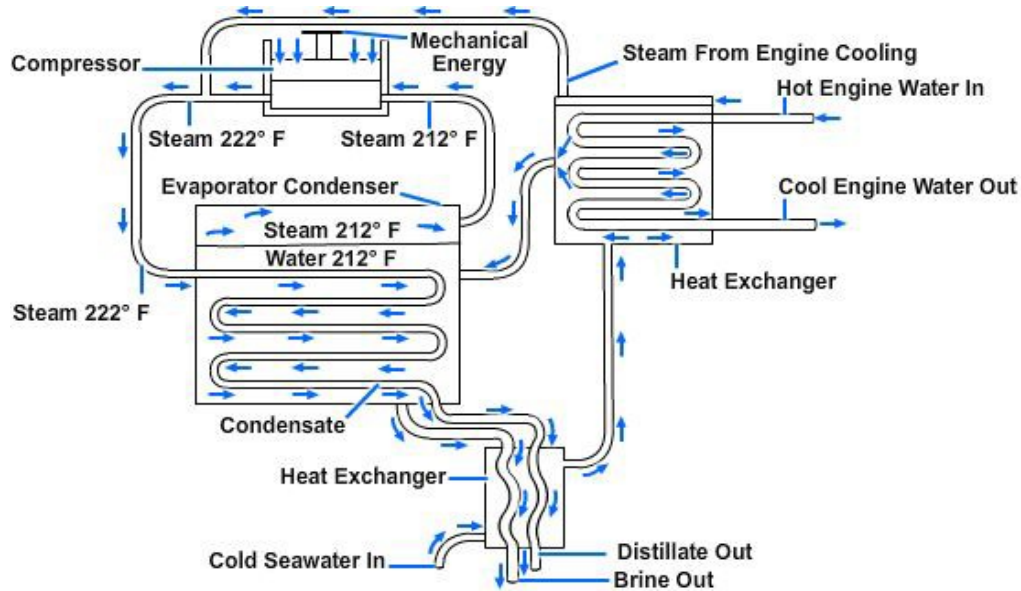
Figure 5-11 — Flow diagram-thermocompression distillation.
